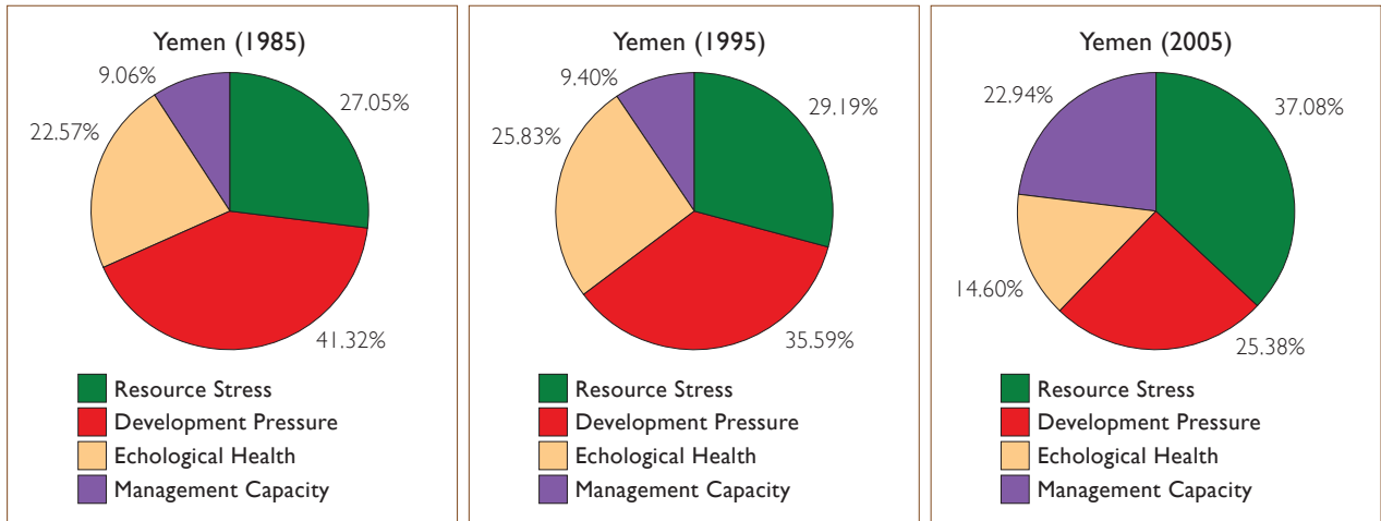
Figure 44: Share of the parameters group to the final Vulnerability Index for Yemen
