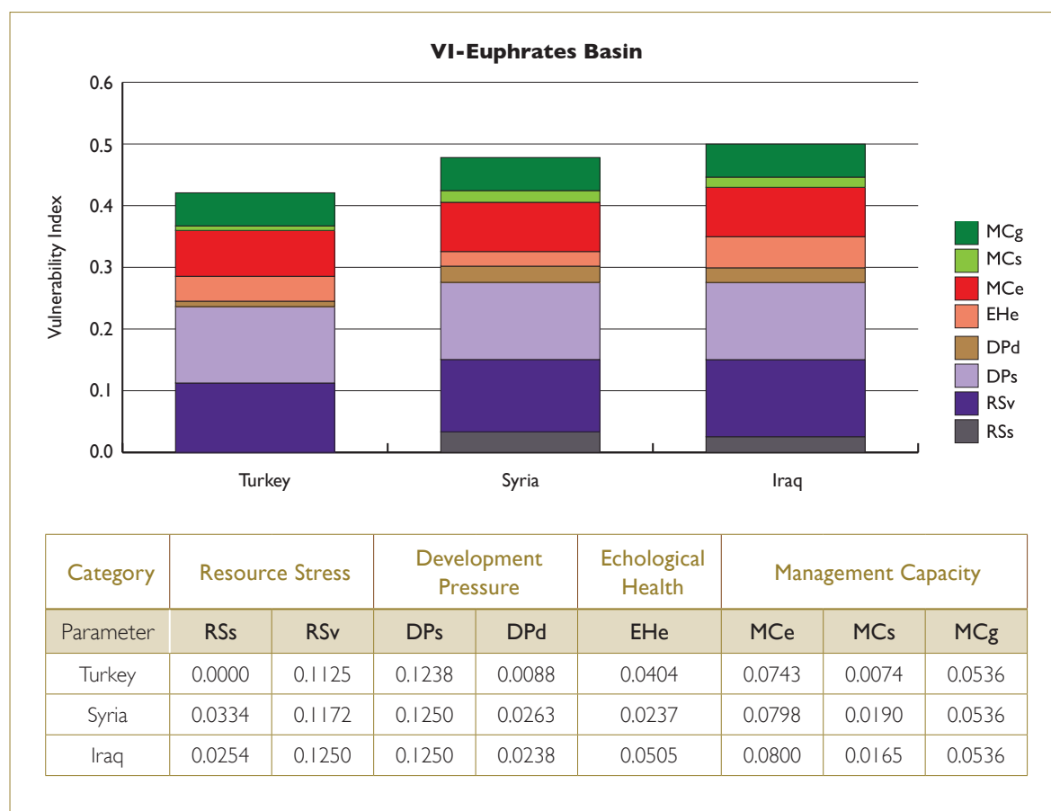
Figure 60: Vulnerability of Euphrates basin
