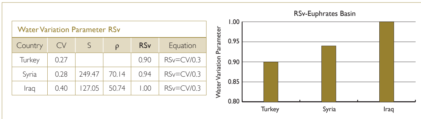
Figure 51: Water variation for the year 2000
